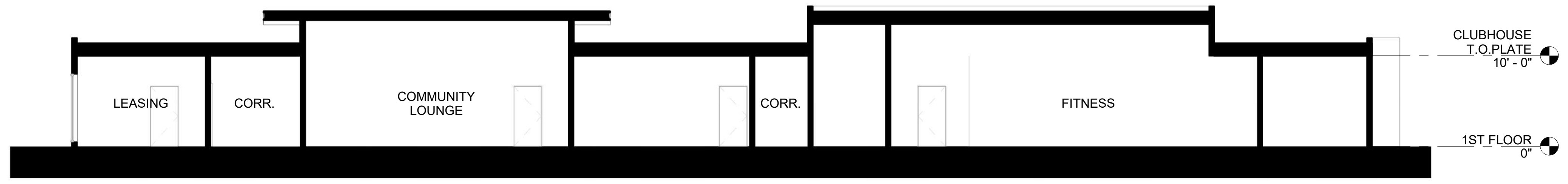
CLUBHOUSE SECTION 1 1/8" = 1'-0"
