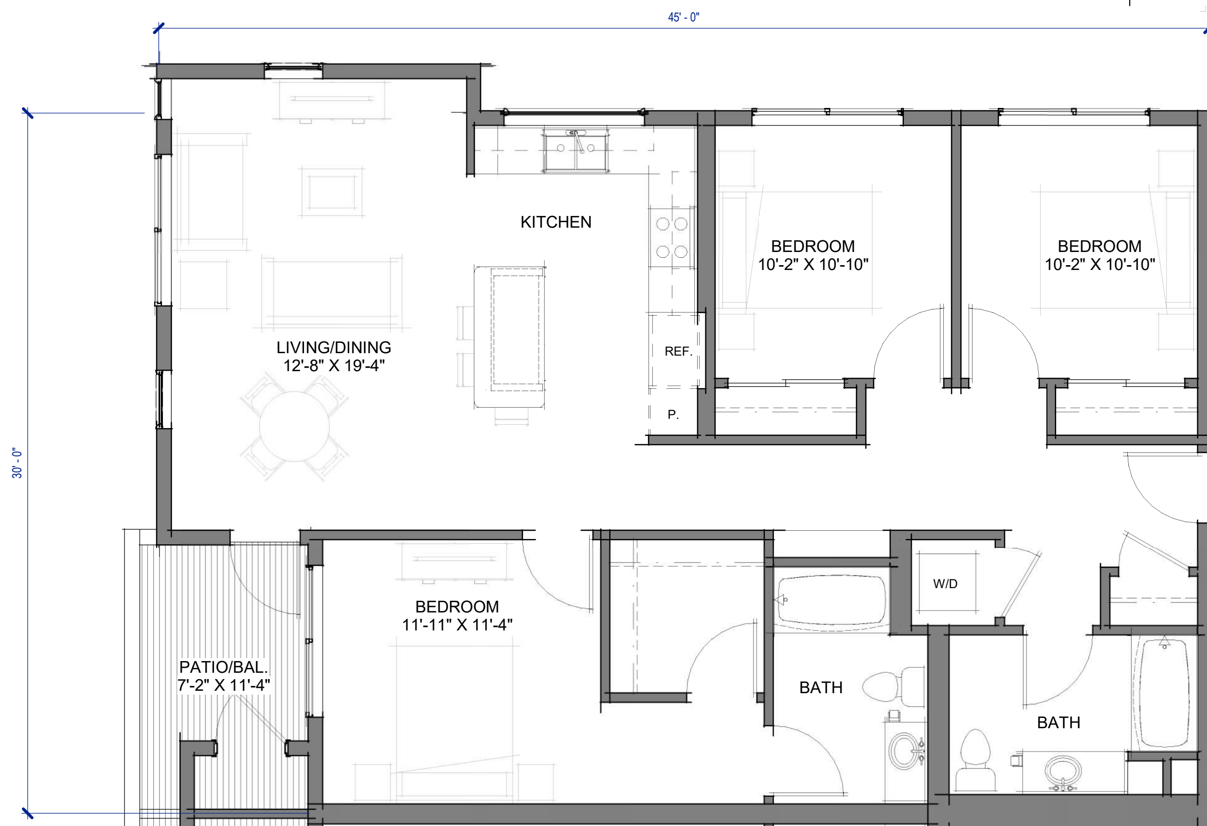
UNIT C1 - 1,302 SF 1/4" = 1'-0" 4
